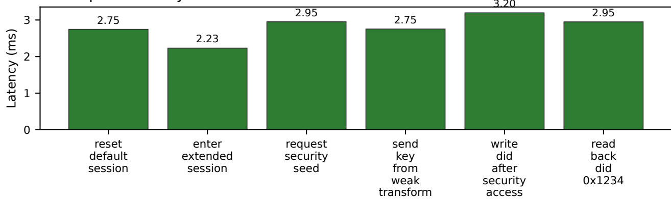
Per-request latency
