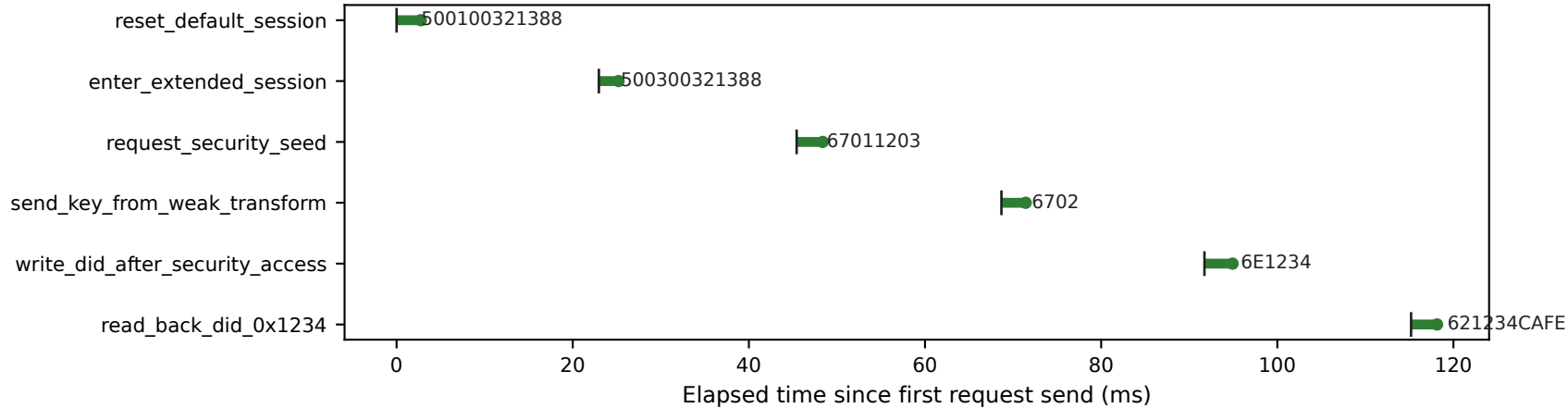
Per-request latency
